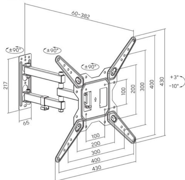
Dimensions (mm)
